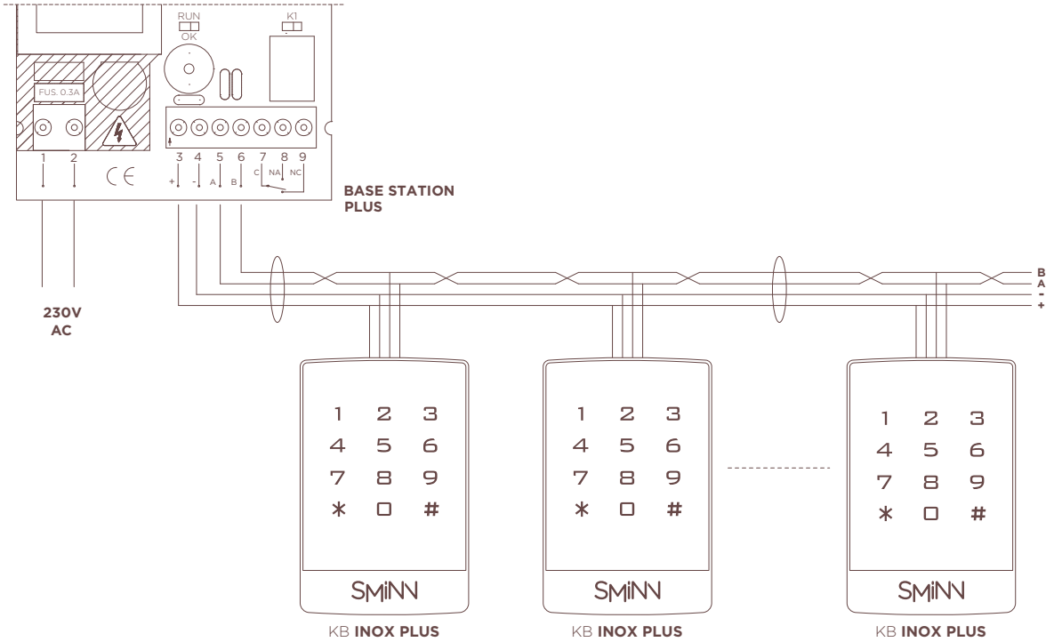
Fig. 2 BUS connection
